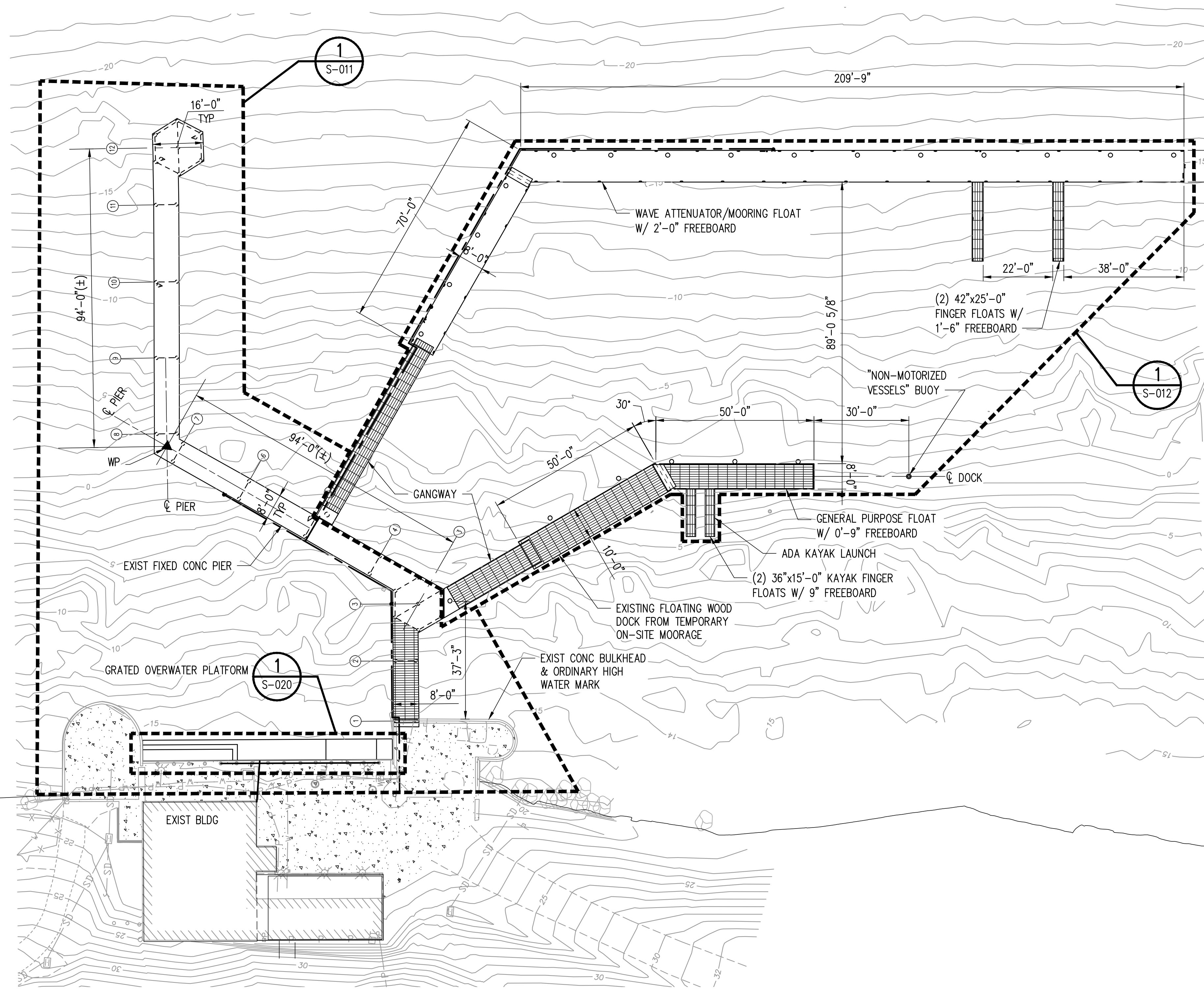
PIER PLAN 0 20 40 60 SCALE IN FEET
